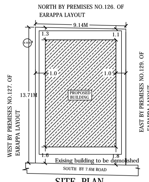
SITE PLAN
